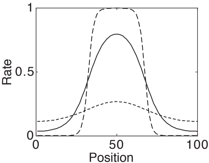
Activity profile at t = 20 \tau
