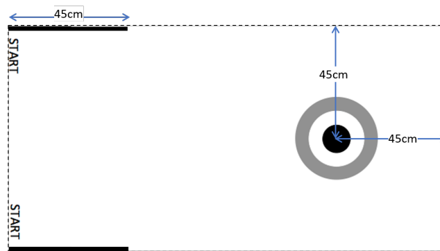
Figure 2: The robot curling sheet.
