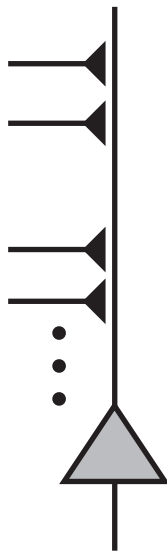
B. Clustered voltage-dependent synapses
